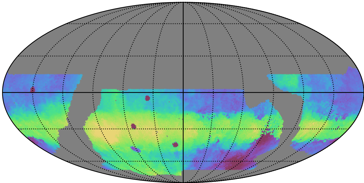
baseline_v2.1_10yrs WFD r band: Median HA
