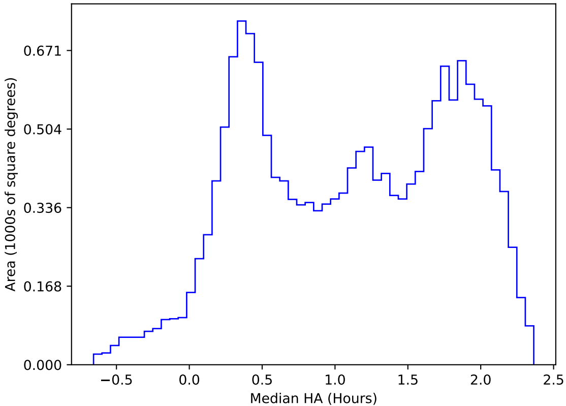
baseline_v2.1_10yrs WFD i band: Median HA
