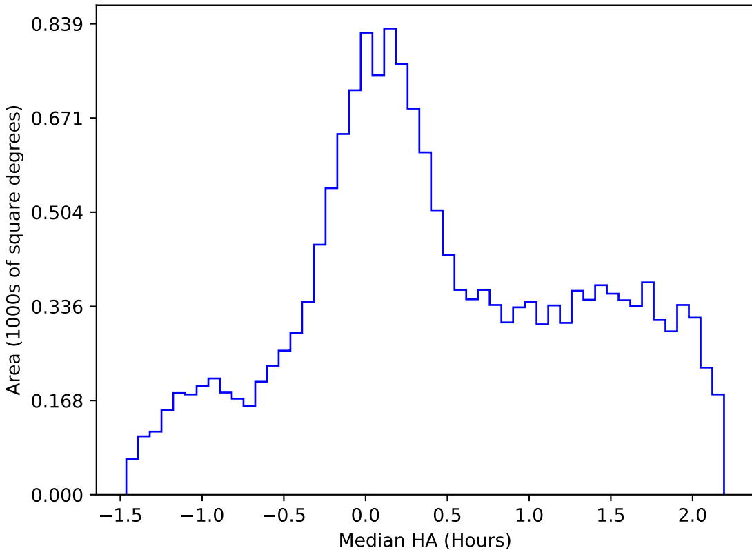
baseline_v2.1_10yrs WFD g band: Median HA
