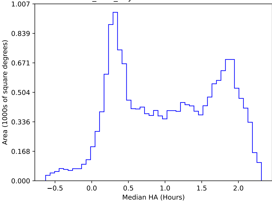
baseline_v2.1_10yrs WFD all bands: Median HA
