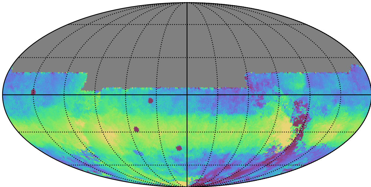
baseline_v2.1_10yrs All sky y band: Median HA
