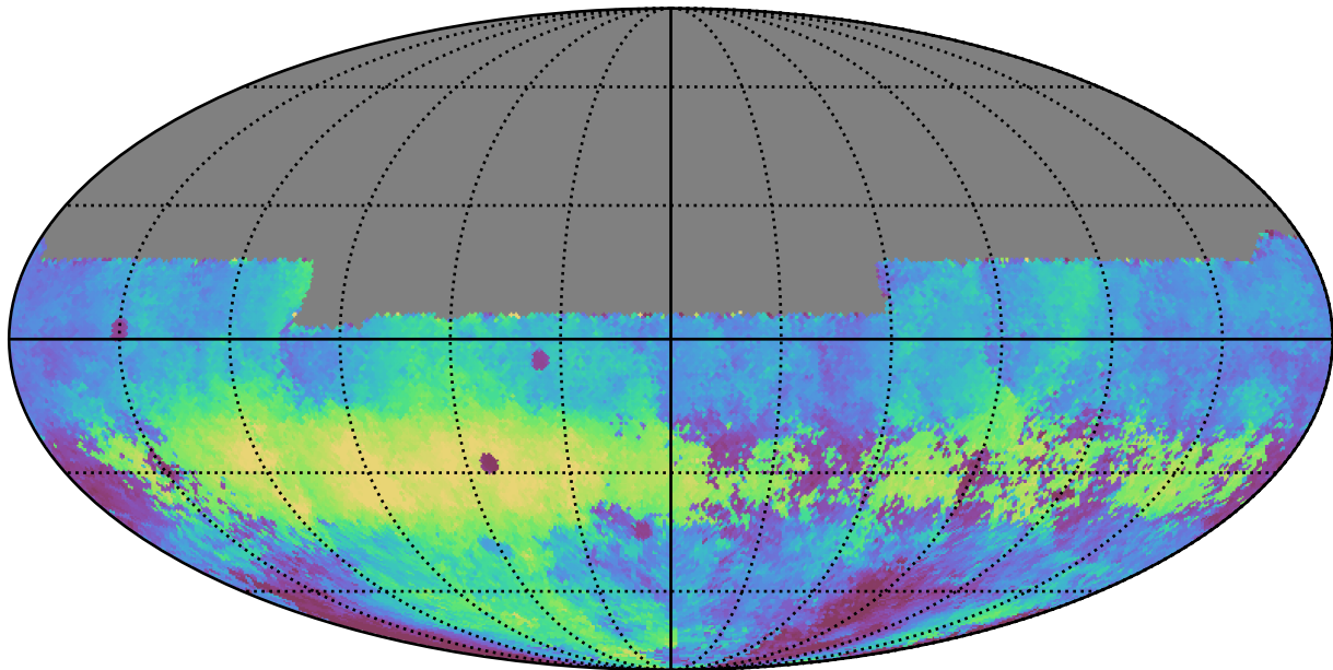
baseline_v2.1_10yrs All sky u band: Median HA
