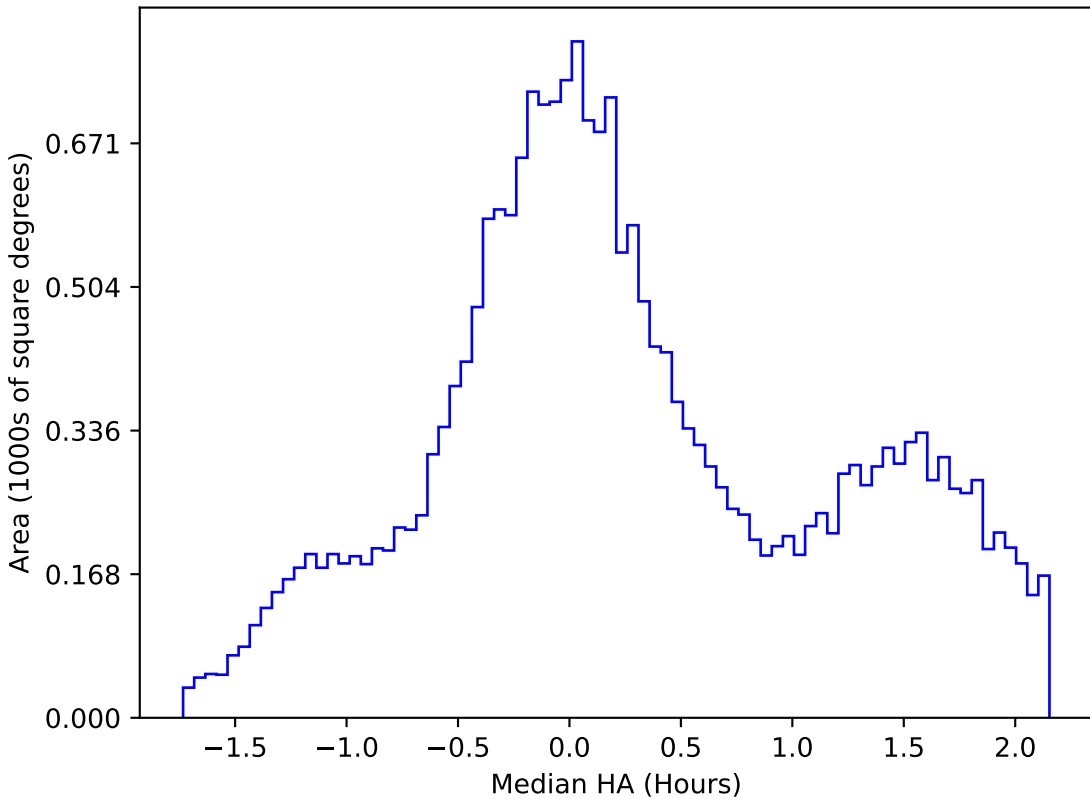
baseline_v2.1_10yrs All sky u band: Median HA
