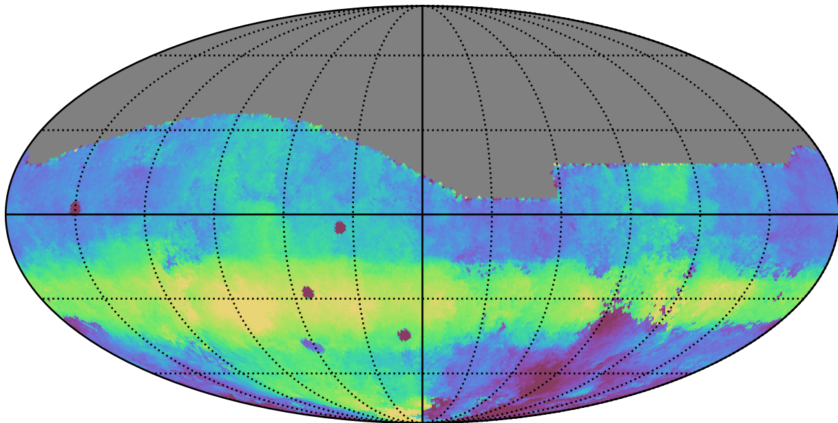
baseline_v2.1_10yrs All sky r band: Median HA
