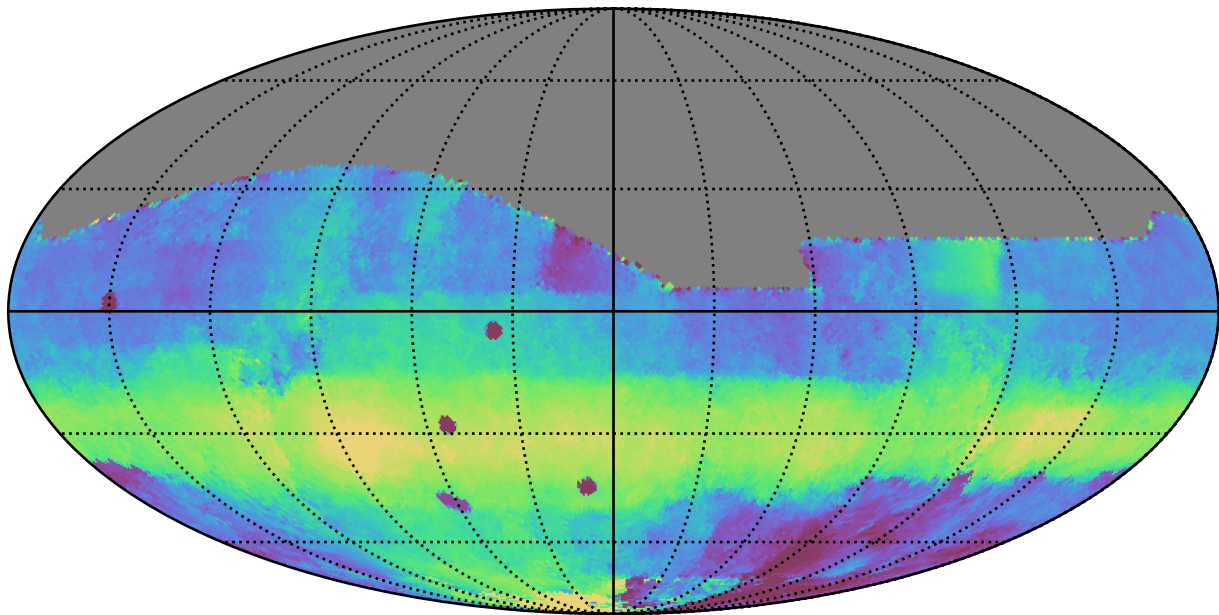
baseline_v2.1_10yrs All sky i band: Median HA
