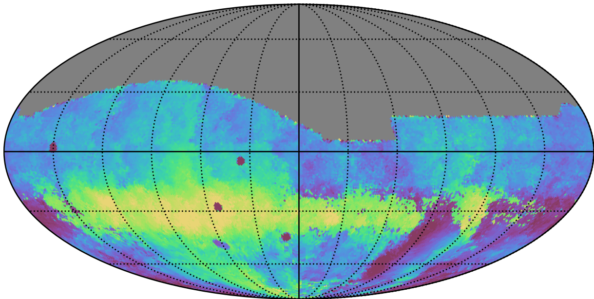
baseline_v2.1_10yrs All sky g band: Median HA
