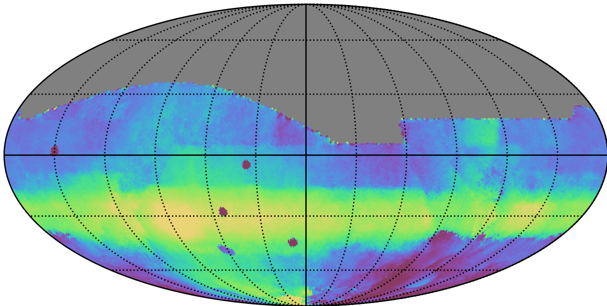
baseline_v2.1_10yrs All sky all bands: Median HA
