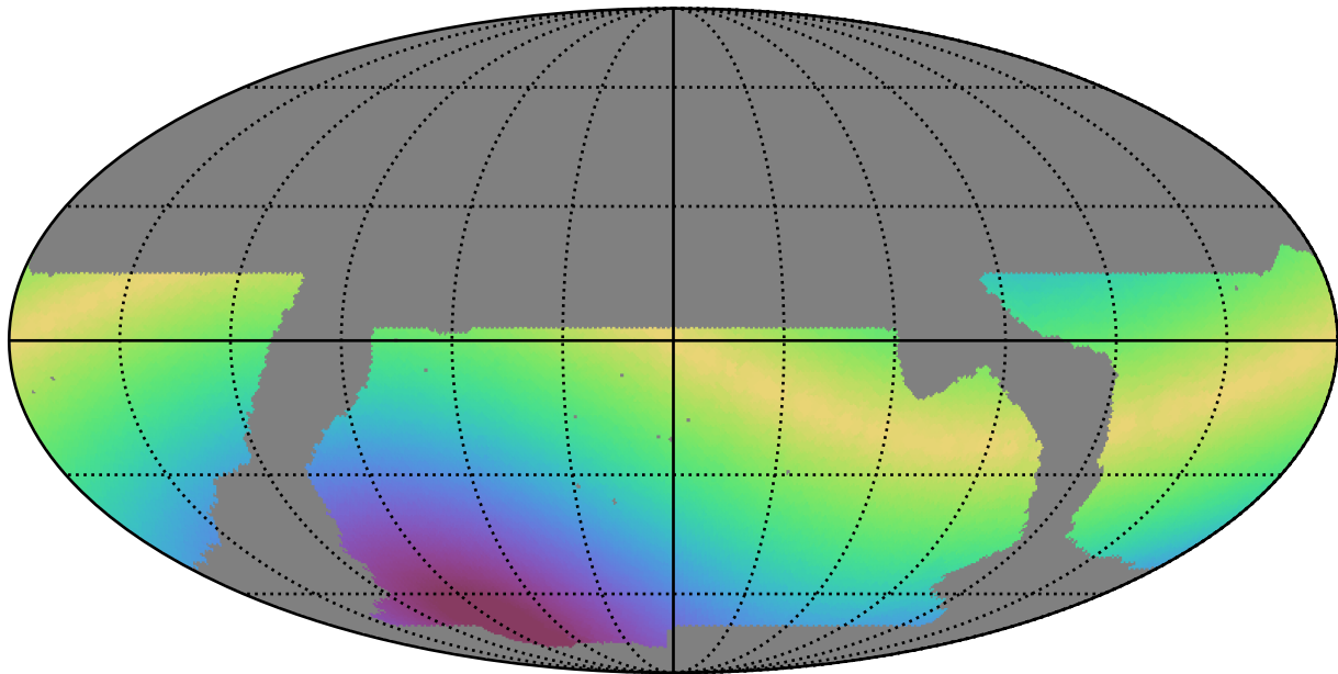
baseline_v2.1_10yrs WFD z band: Max solarElong
