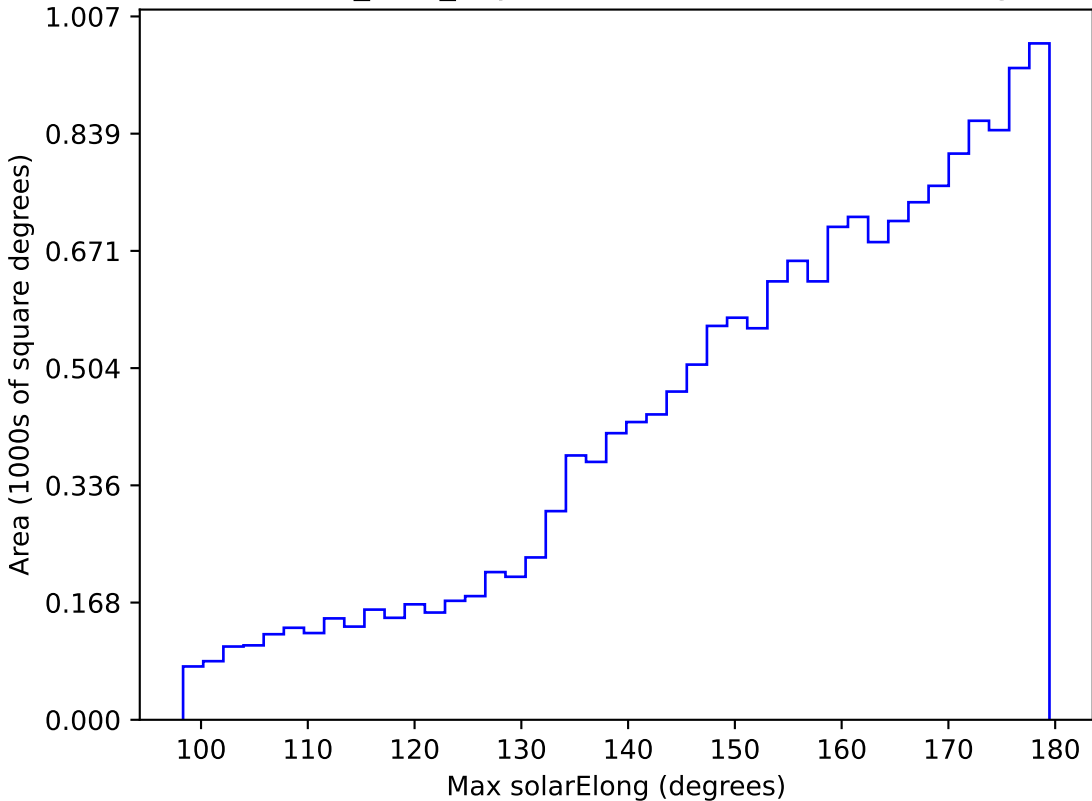
baseline_v2.1_10yrs WFD z band: Max solarElong
