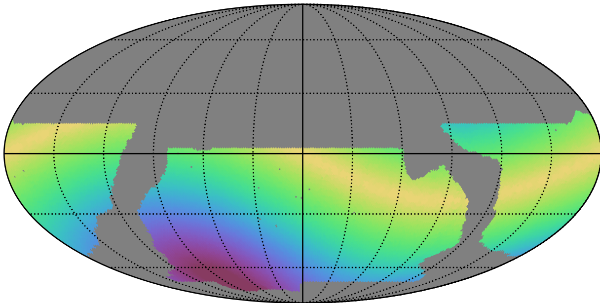
baseline_v2.1_10yrs WFD r band: Max solarElong
