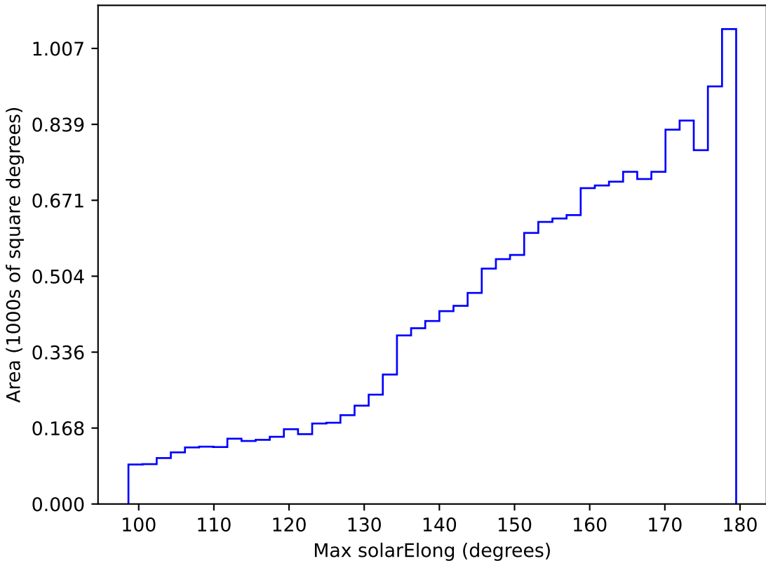
baseline_v2.1_10yrs WFD r band: Max solarElong
