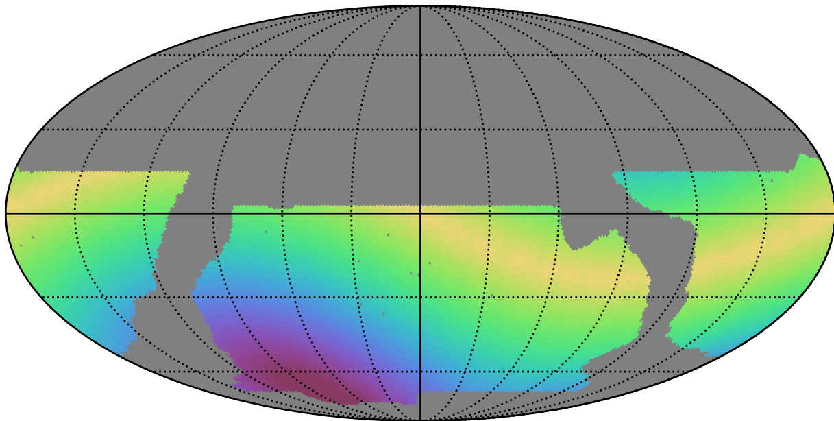
baseline_v2.1_10yrs WFD g band: Max solarElong
