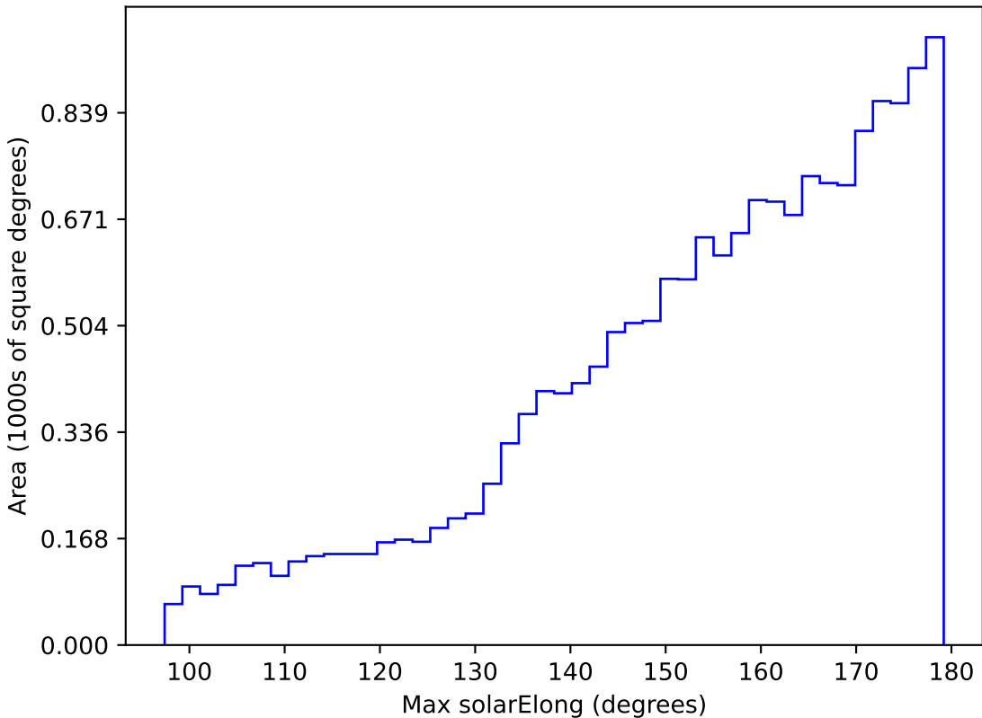
baseline_v2.1_10yrs WFD g band: Max solarElong
