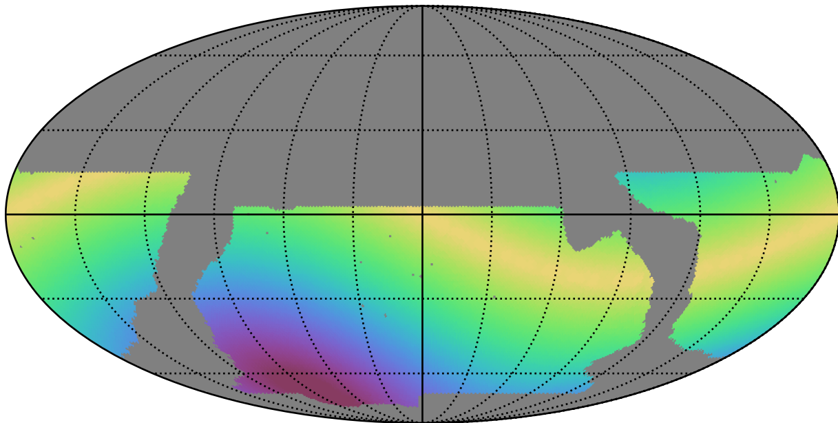
baseline_v2.1_10yrs WFD all bands: Max solarElong
