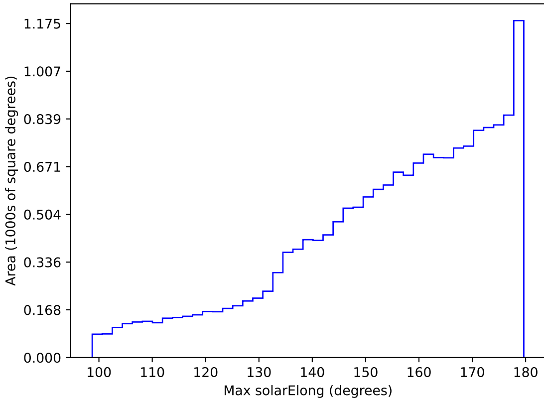
baseline_v2.1_10yrs WFD all bands: Max solarElong
