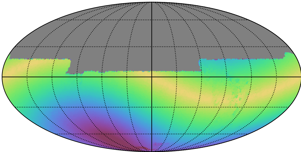
baseline_v2.1_10yrs All sky y band: Max solarElong
