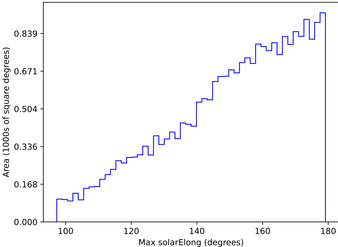
baseline_v2.1_10yrs All sky y band: Max solarElong
