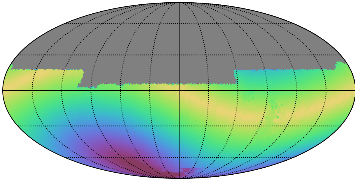
baseline_v2.1_10yrs All sky u band: Max solarElong
