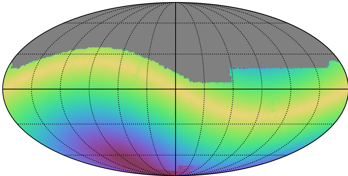
baseline_v2.1_10yrs All sky r band: Max solarElong
