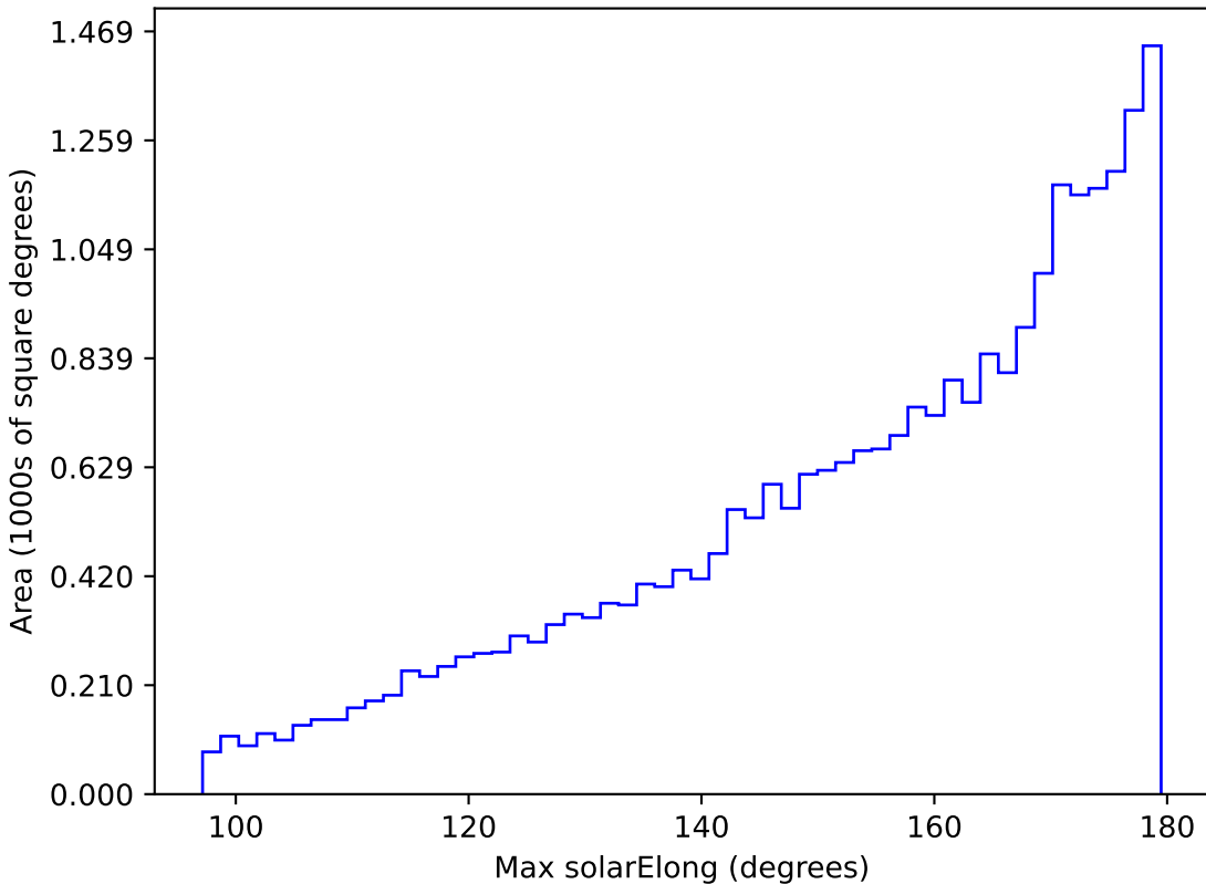
baseline_v2.1_10yrs All sky r band: Max solarElong
