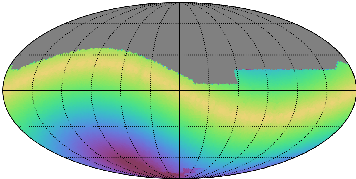
baseline_v2.1_10yrs All sky g band: Max solarElong
