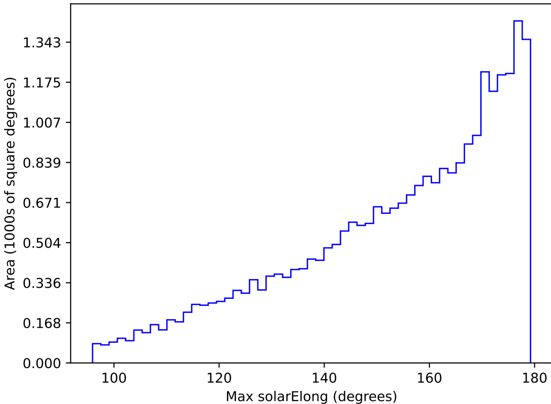
baseline_v2.1_10yrs All sky g band: Max solarElong
