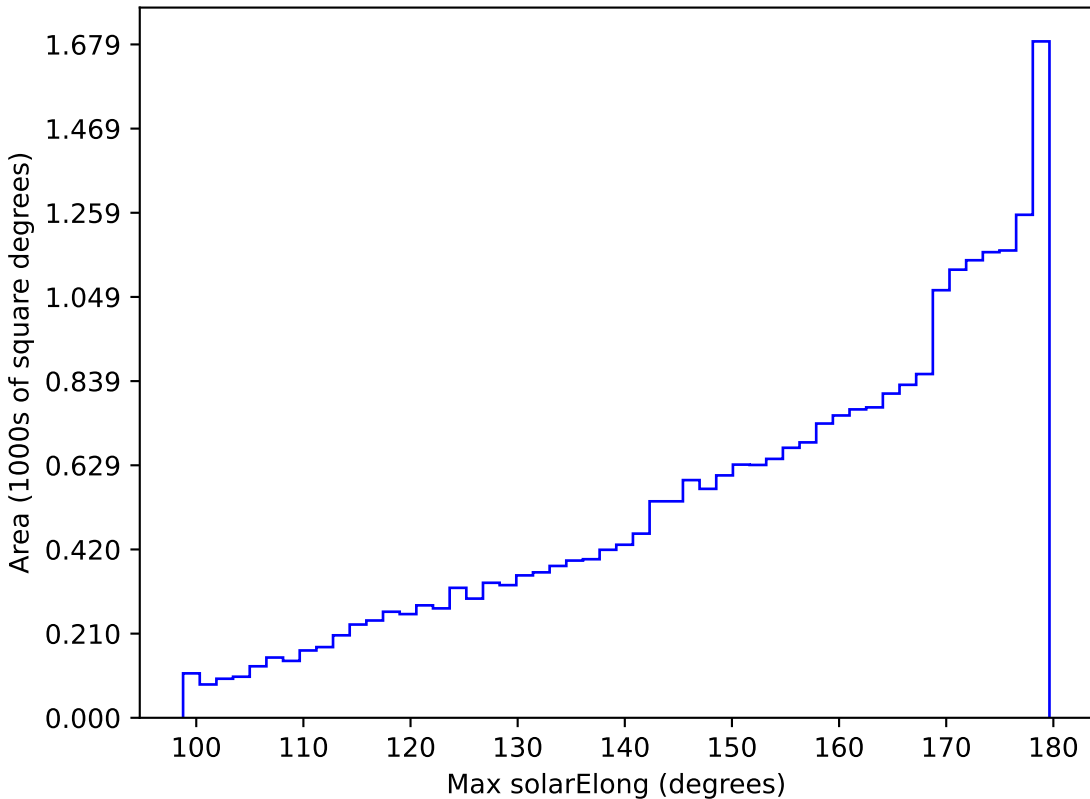
baseline_v2.1_10yrs All sky all bands: Max solarElong
