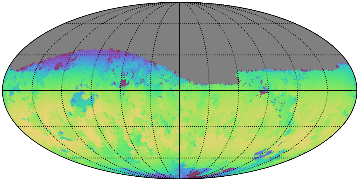
baseline_v2.1_10yrs Yr 1 z band: Max skyBrightness
