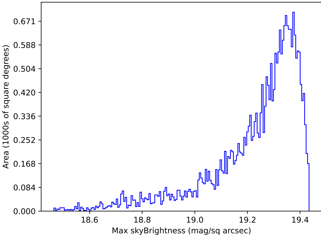
baseline_v2.1_10yrs Yr 1 z band: Max skyBrightness
