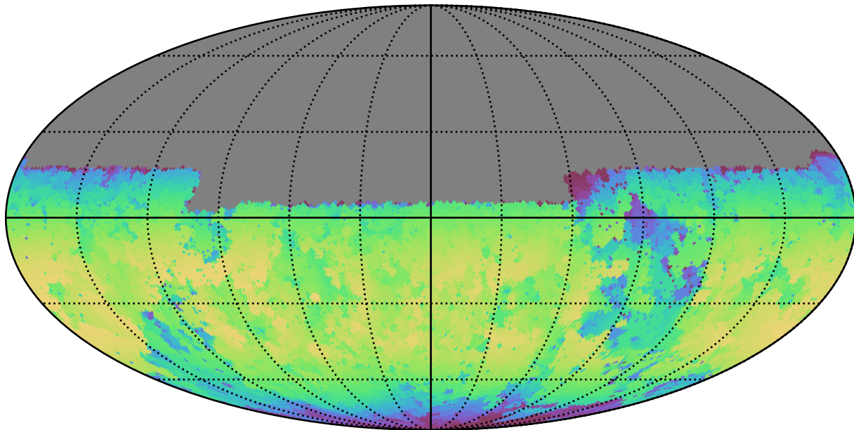
baseline_v2.1_10yrs Yr 1 y band: Max skyBrightness
