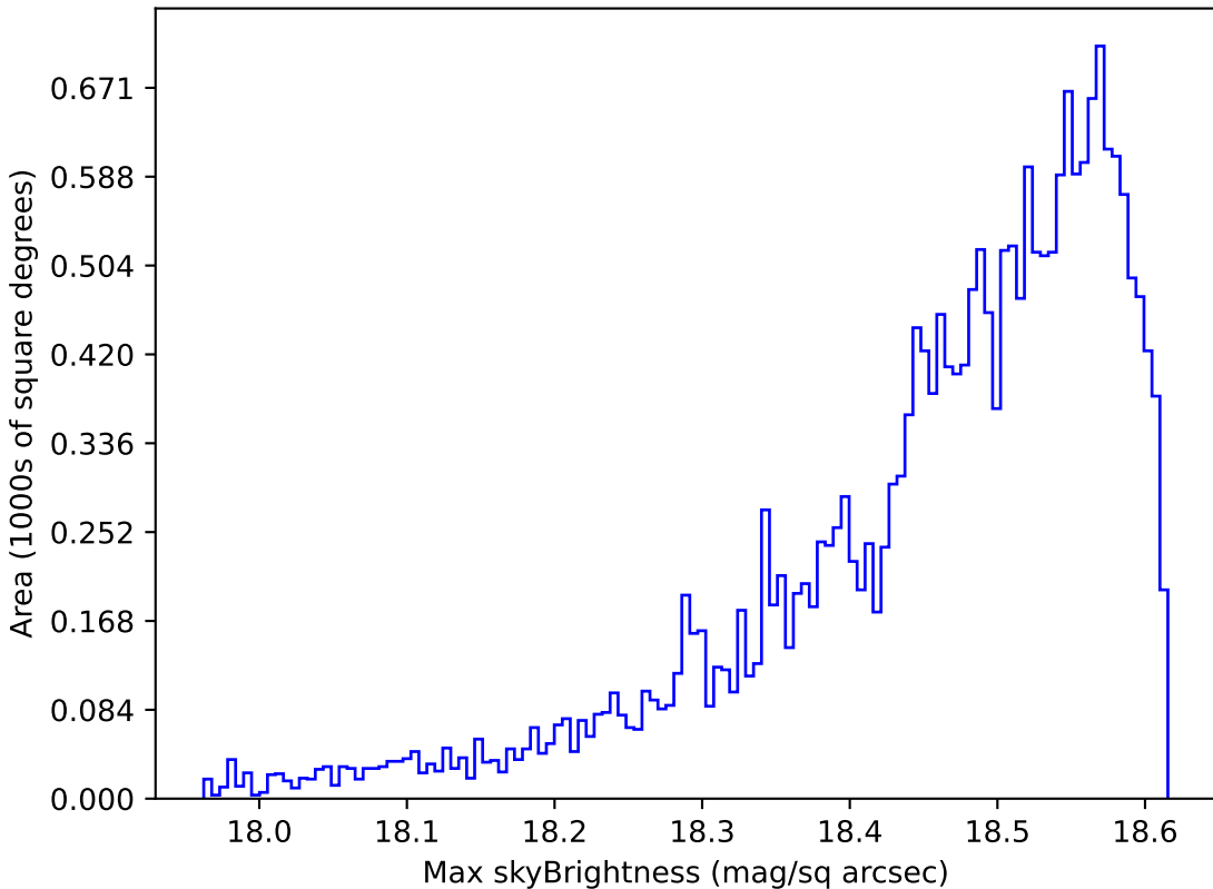
baseline_v2.1_10yrs Yr 1 y band: Max skyBrightness
