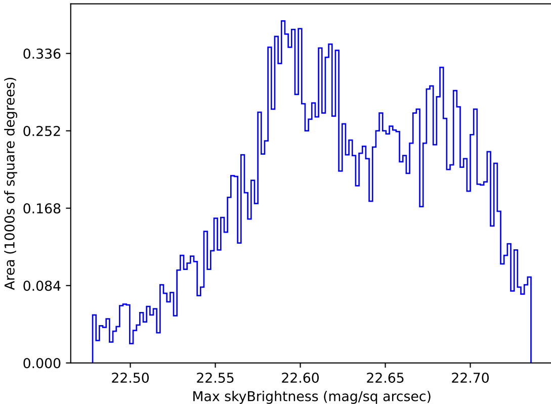
baseline_v2.1_10yrs Yr 1 u band: Max skyBrightness
