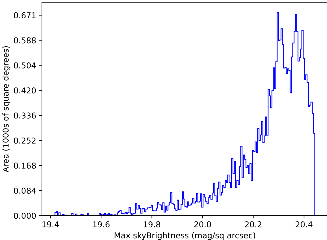
baseline_v2.1_10yrs Yr 1 i band: Max skyBrightness
