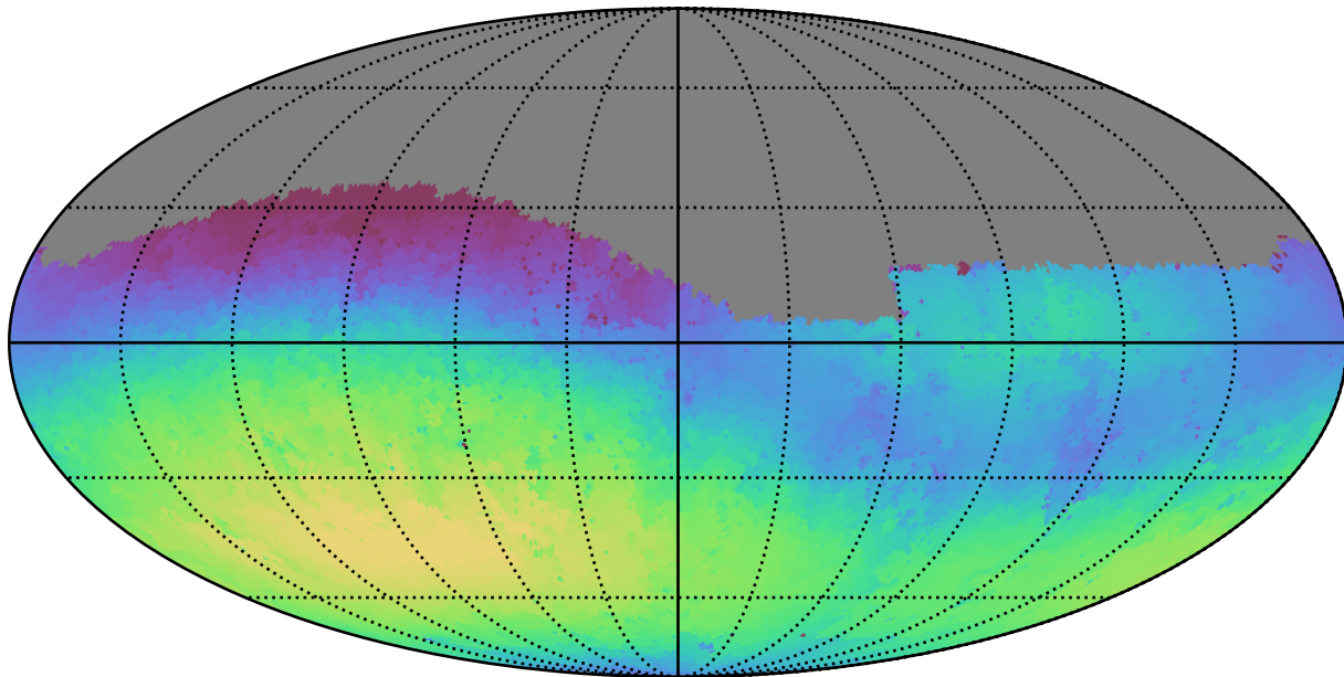
baseline_v2.1_10yrs Yr 1 g band: Max skyBrightness
