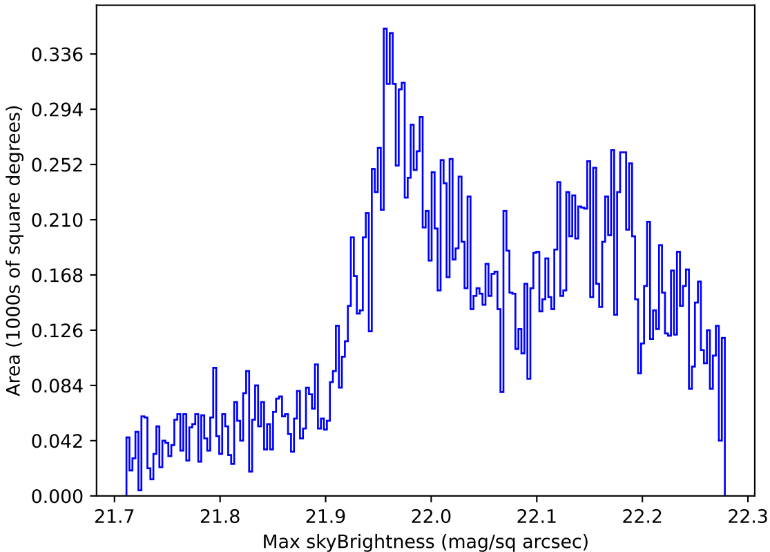
baseline_v2.1_10yrs Yr 1 g band: Max skyBrightness
