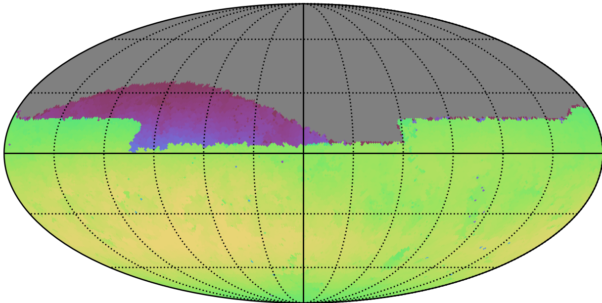
baseline_v2.1_10yrs Yr 1 all bands: Max skyBrightness
