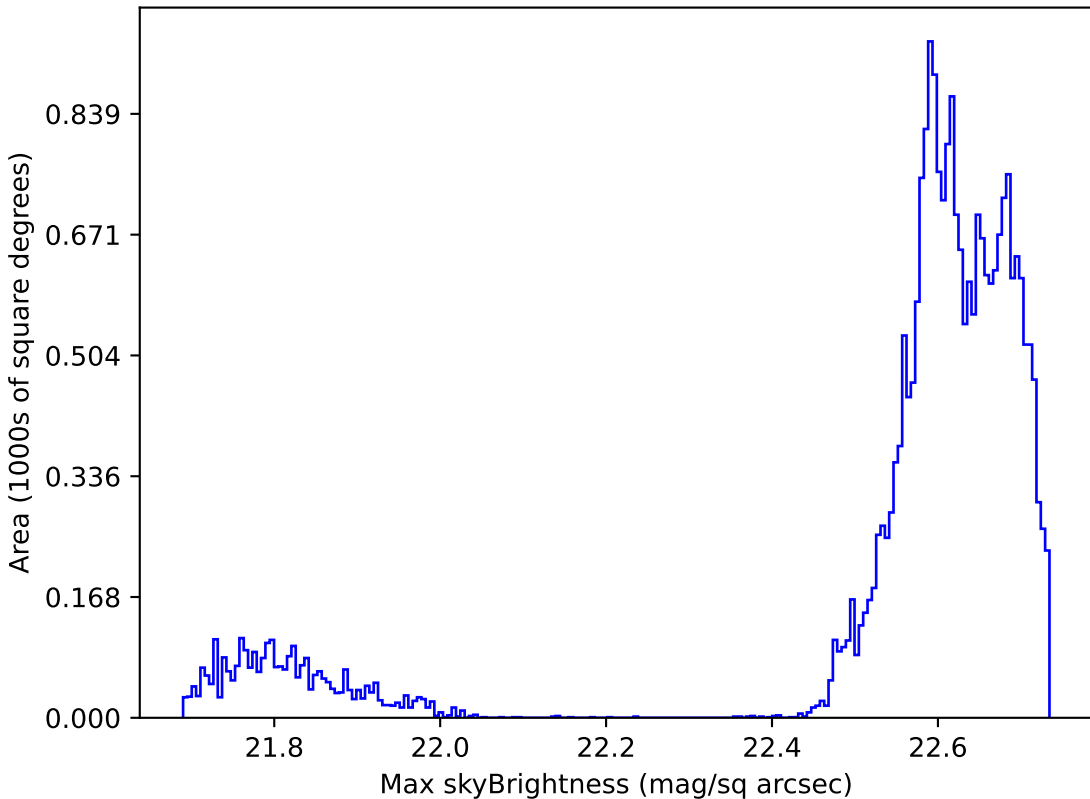
baseline_v2.1_10yrs Yr 1 all bands: Max skyBrightness
