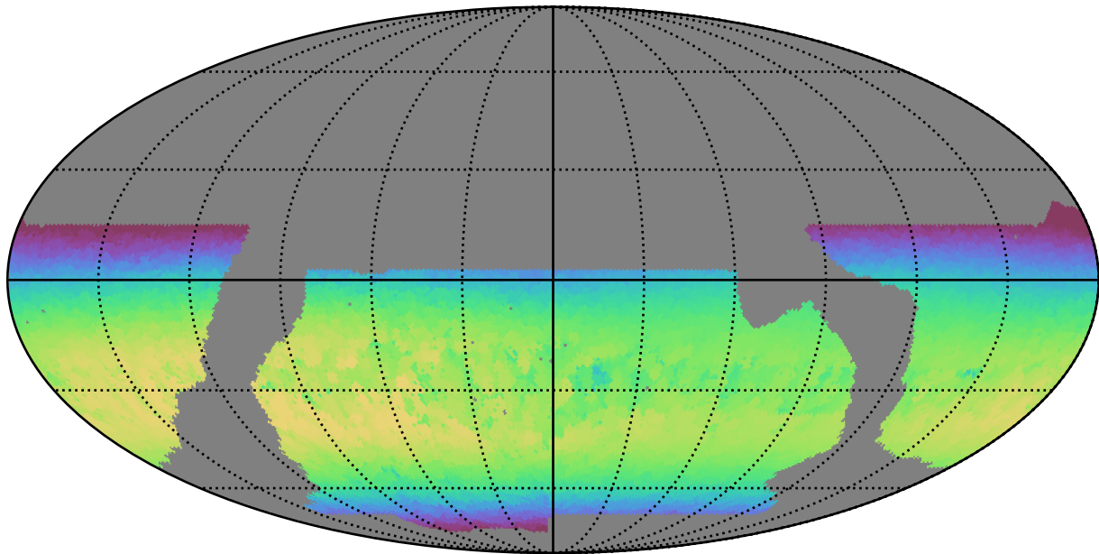
baseline_v2.1_10yrs WFD z band: Max skyBrightness
