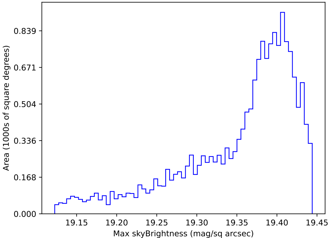
baseline_v2.1_10yrs WFD z band: Max skyBrightness
