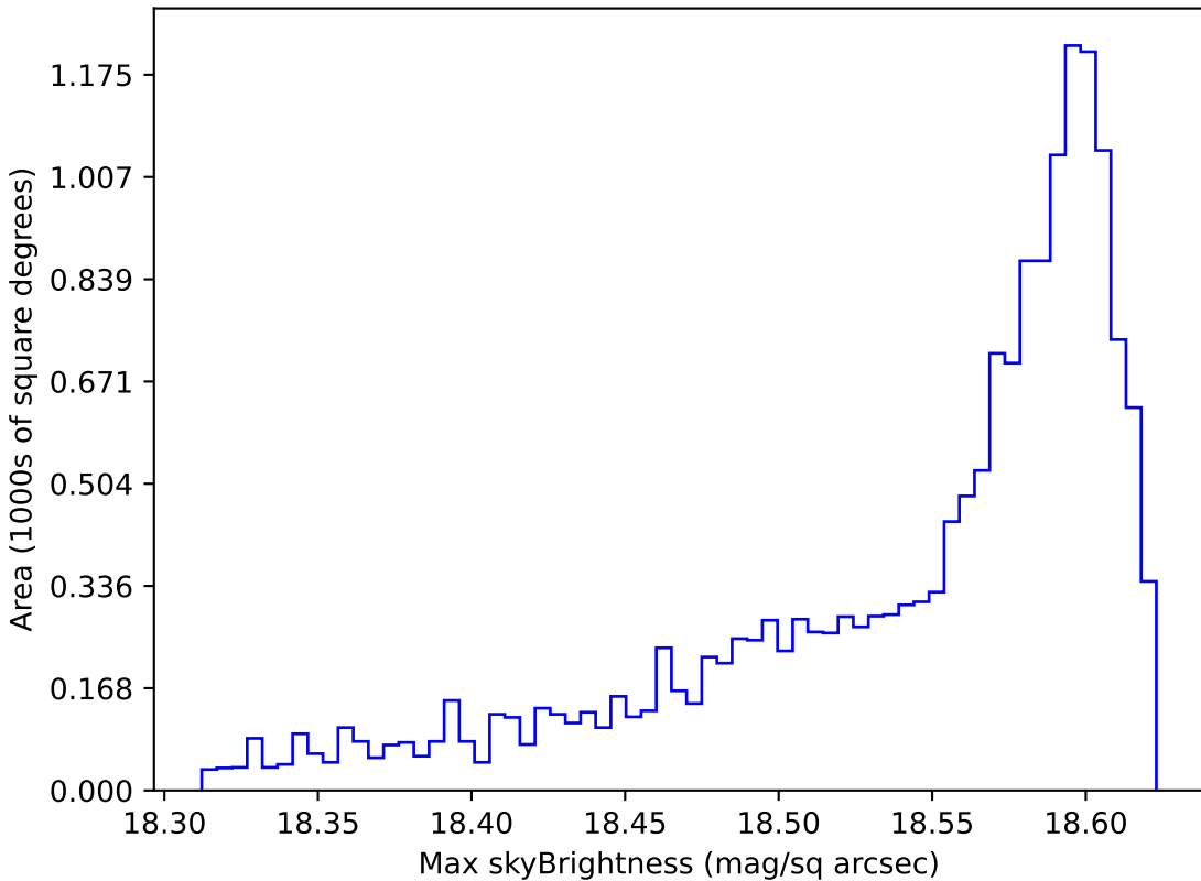
baseline_v2.1_10yrs WFD y band: Max skyBrightness
