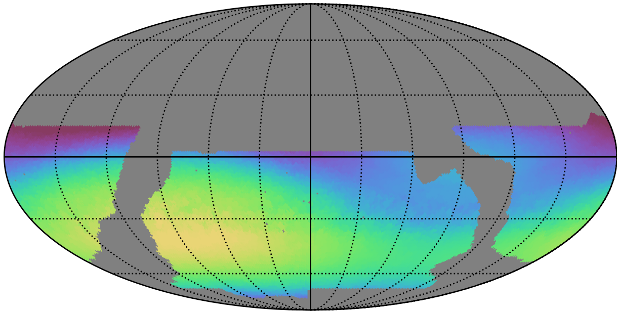
baseline_v2.1_10yrs WFD r band: Max skyBrightness
