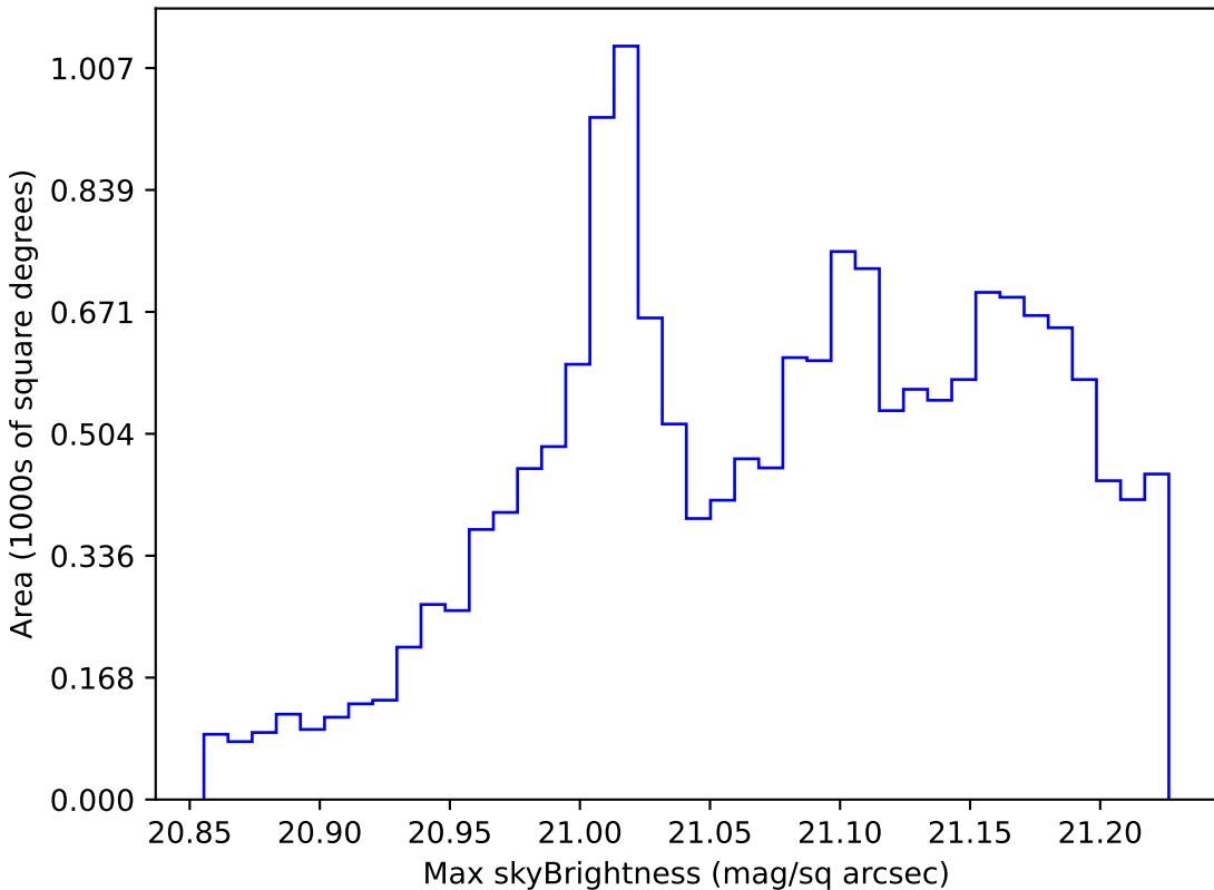
baseline_v2.1_10yrs WFD r band: Max skyBrightness
