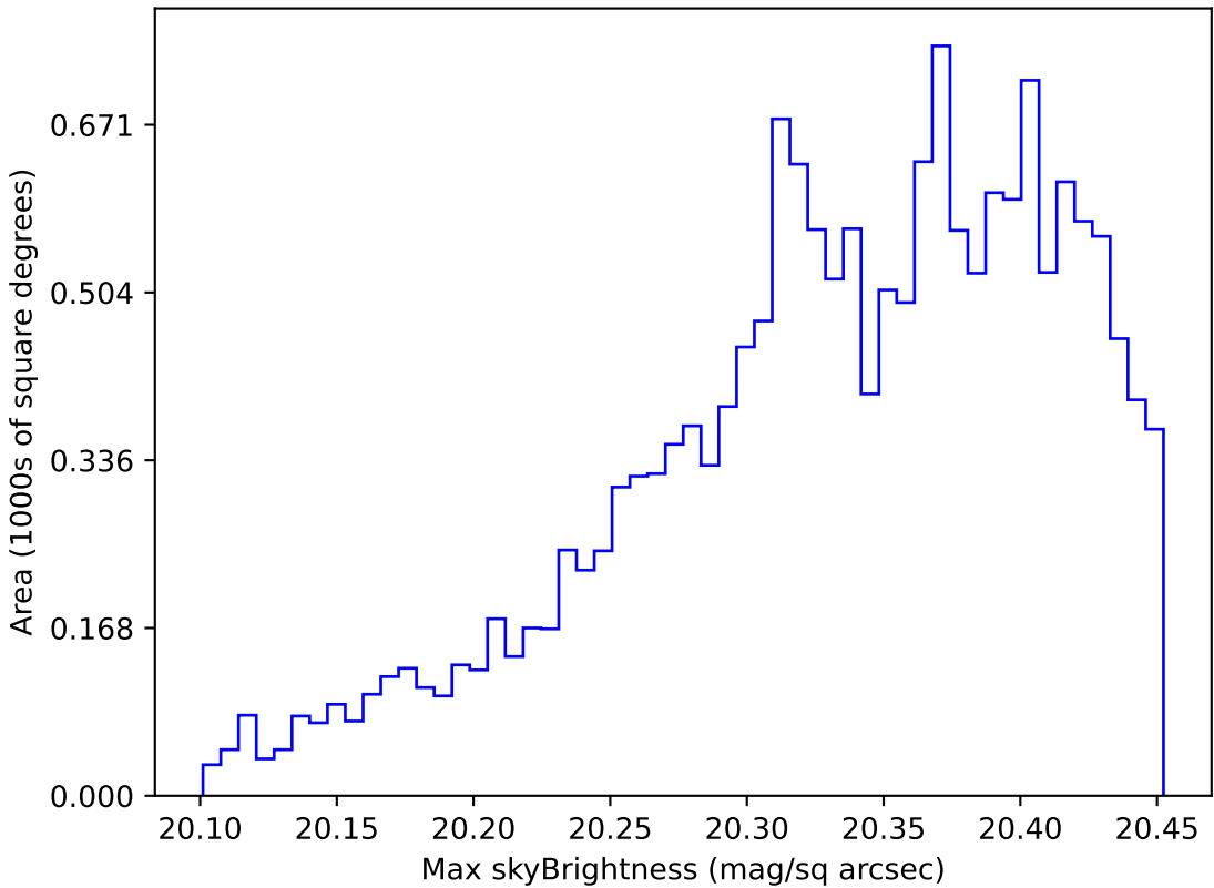
baseline_v2.1_10yrs WFD i band: Max skyBrightness
