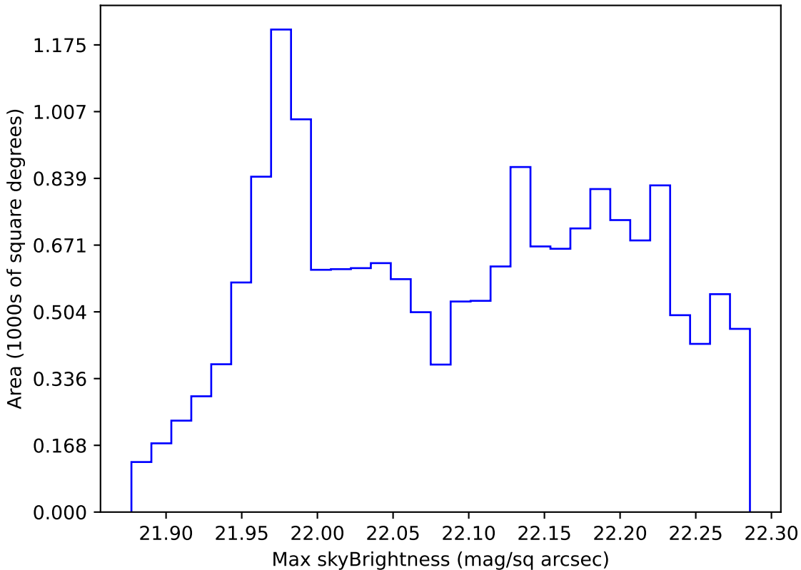
baseline_v2.1_10yrs WFD g band: Max skyBrightness
