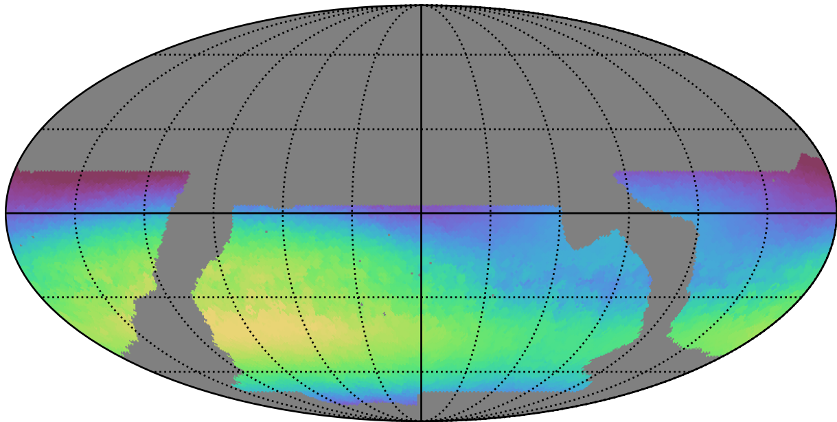
baseline_v2.1_10yrs WFD all bands: Max skyBrightness
