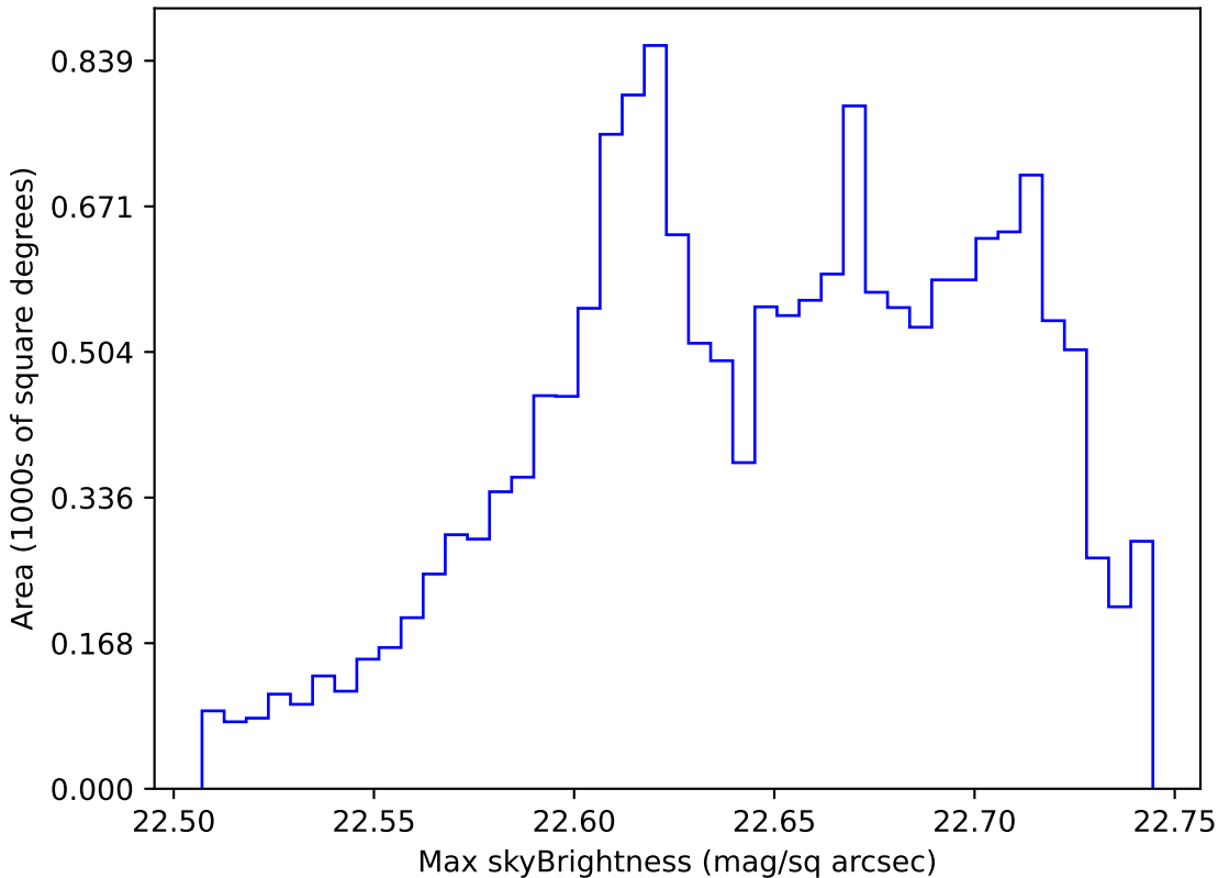
baseline_v2.1_10yrs WFD all bands: Max skyBrightness
