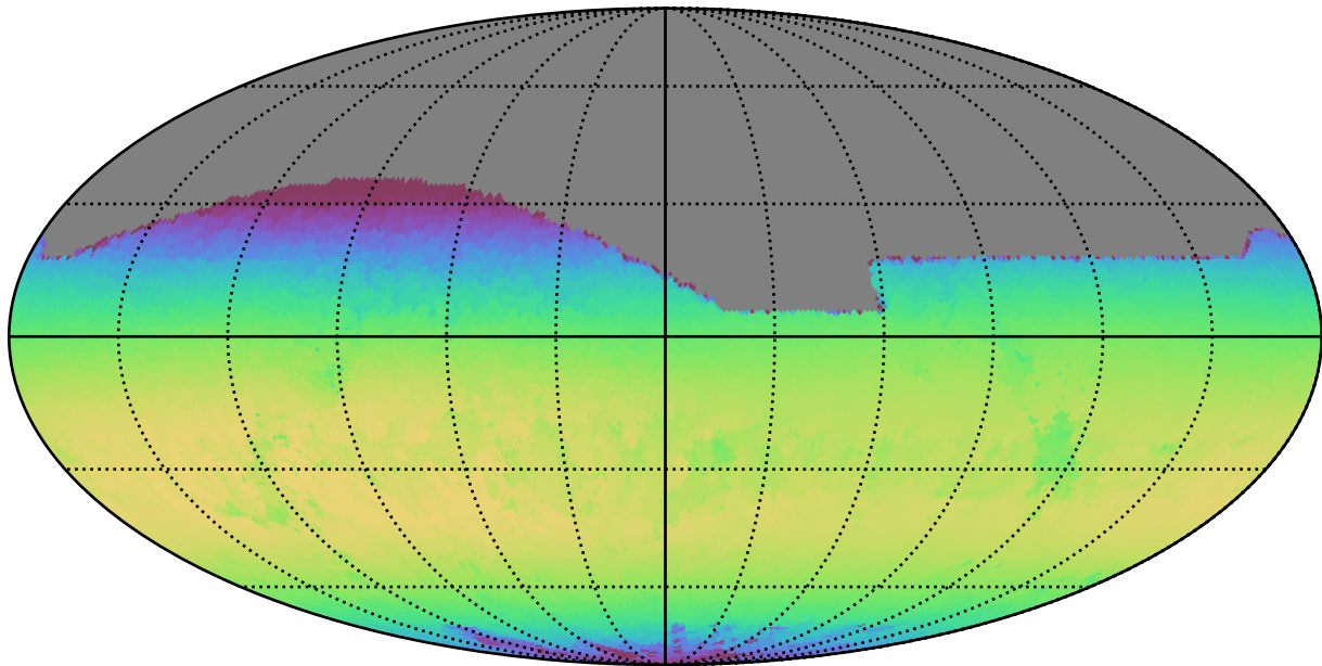
baseline_v2.1_10yrs All sky z band: Max skyBrightness
