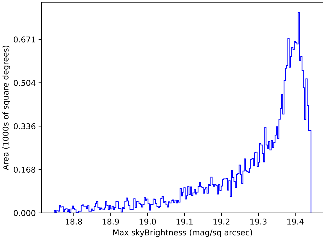
baseline_v2.1_10yrs All sky z band: Max skyBrightness
