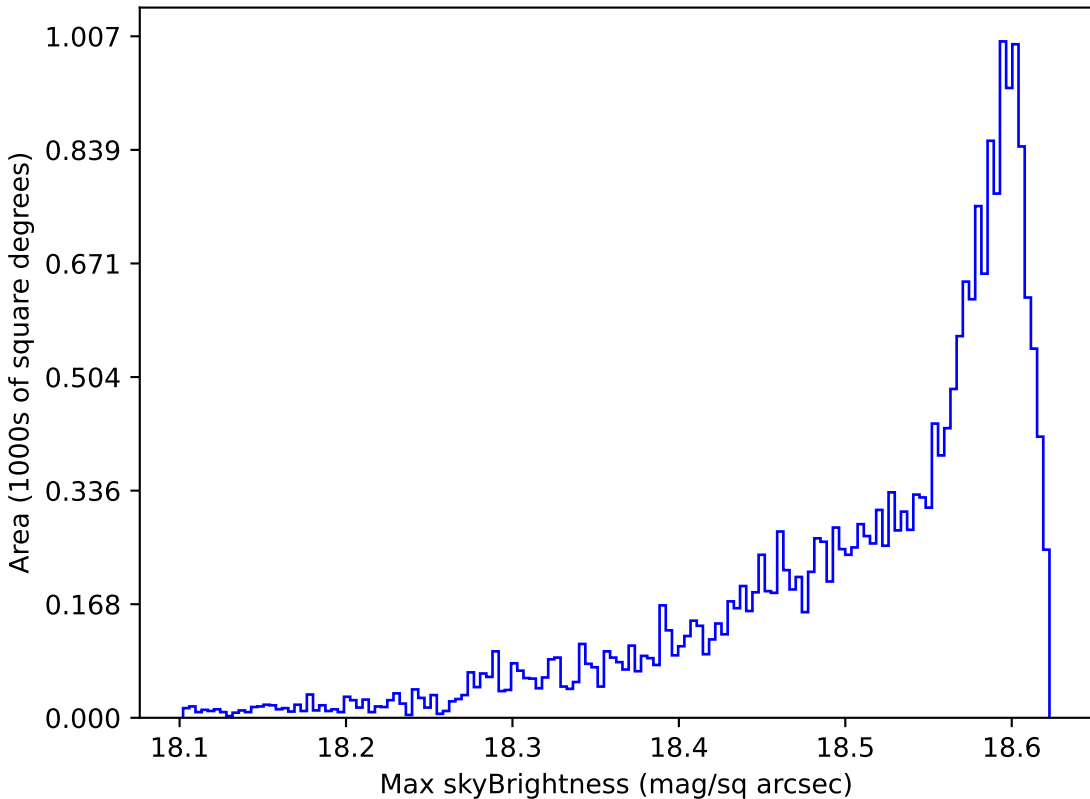
baseline_v2.1_10yrs All sky y band: Max skyBrightness
