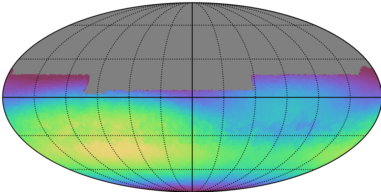
baseline_v2.1_10yrs All sky u band: Max skyBrightness
